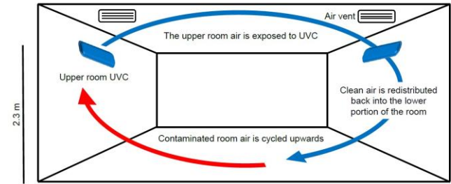
Figure 7. Upper room UVC air disinfection system.
